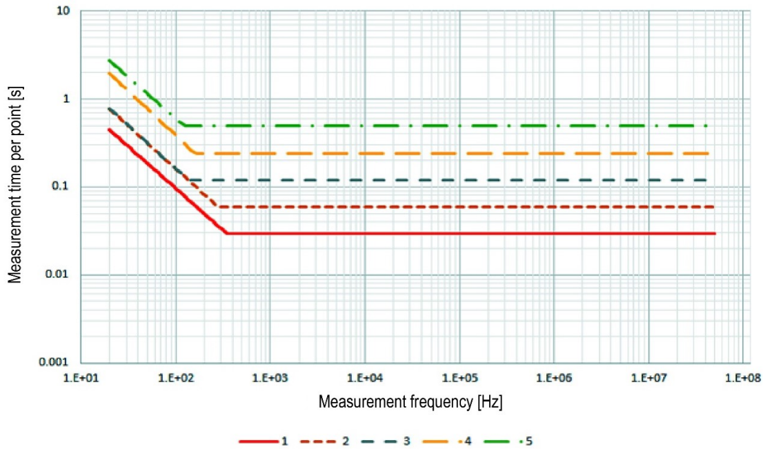
Figure 4. Measurement time (Option 050/ 030/ 020/ 010 without option 001, Typical)
