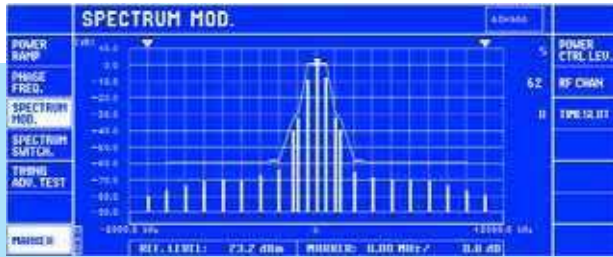
The option CMD-B43 provides measurements of spectrum due to modulation and switching according to GSM recommendations
