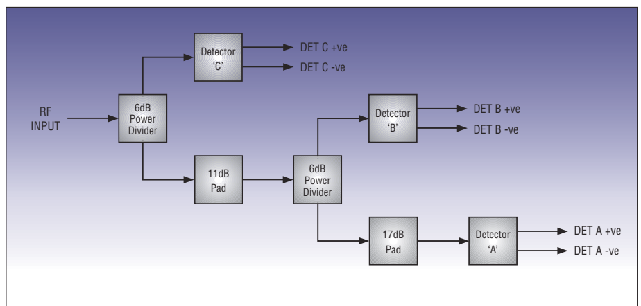
Anritsu's MA2480A series Universal Power Sensors use a unique architecture with three cascaded diode pairs, dividers and attenuators. One of the diode pairs is within its square law region, ensuring true average power measurements of any input signal.
