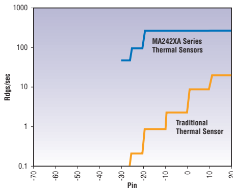
MA2420A/B Thermal Sensors. Rise and fall times of less than 4 ms improve both settling time and measurement rate by more than two orders of magnitude over most of the useful dynamic range.
