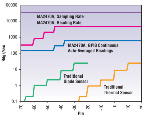
MA2470A Series Power Sensors. 90 dB dynamic range is combined with high speed. Rise time is < 4 µsec. Fall time is < 10 µsec, typical.
